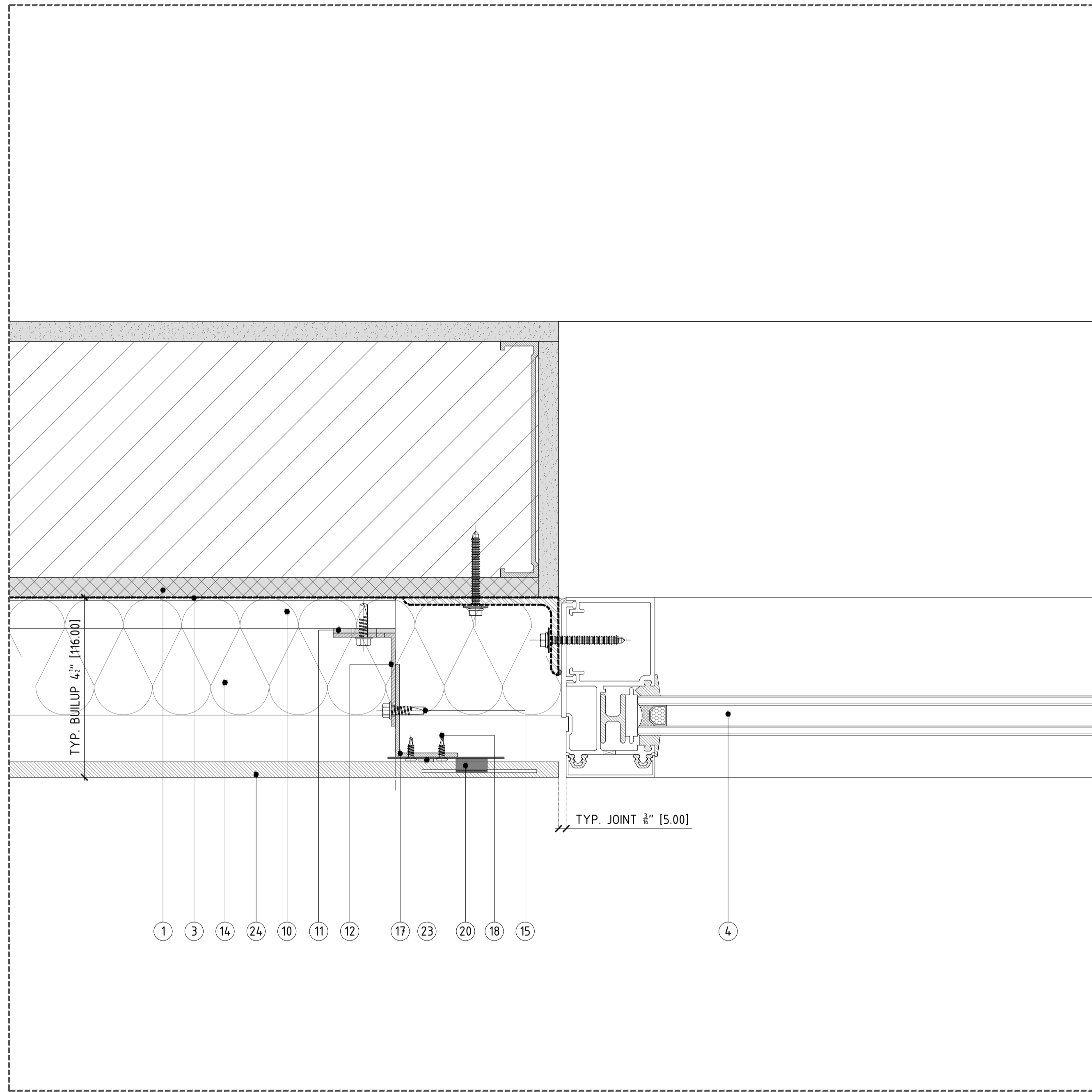
DETAIL A - TYPICAL WINDOW JAMB DETAIL
